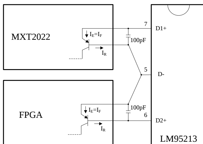
Figure 9-14. Typical Temperature Sensor Application
