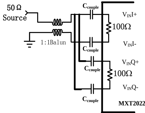
Figure 9-4. Driving DESIQ Mode
