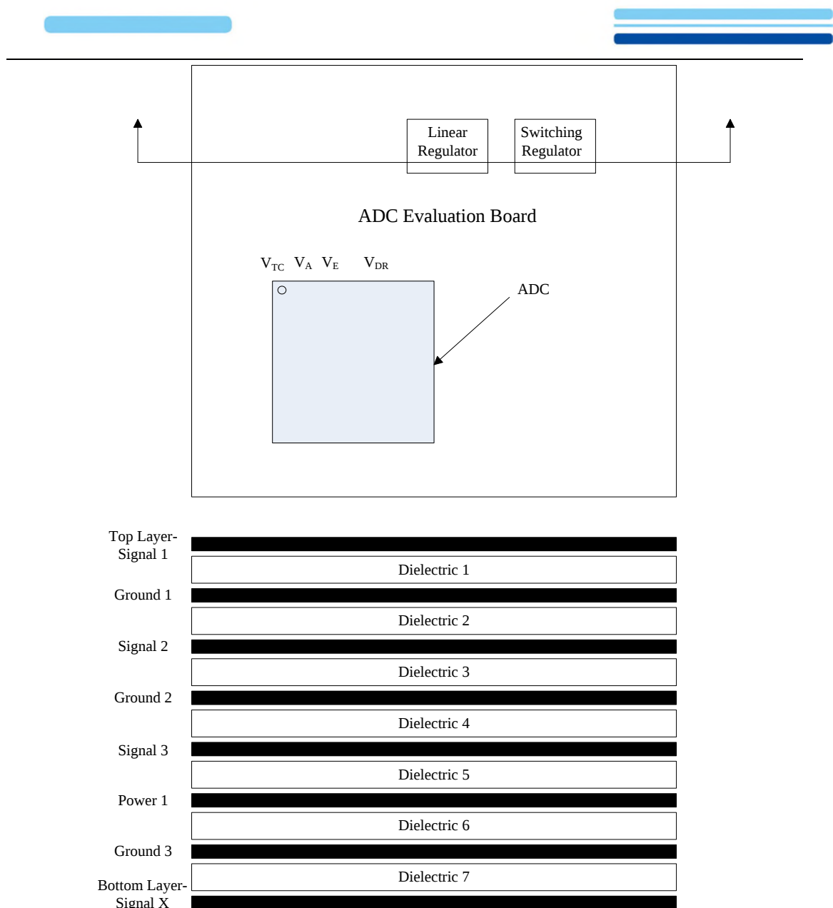
Figure 9-9. Power and Grounding Example
