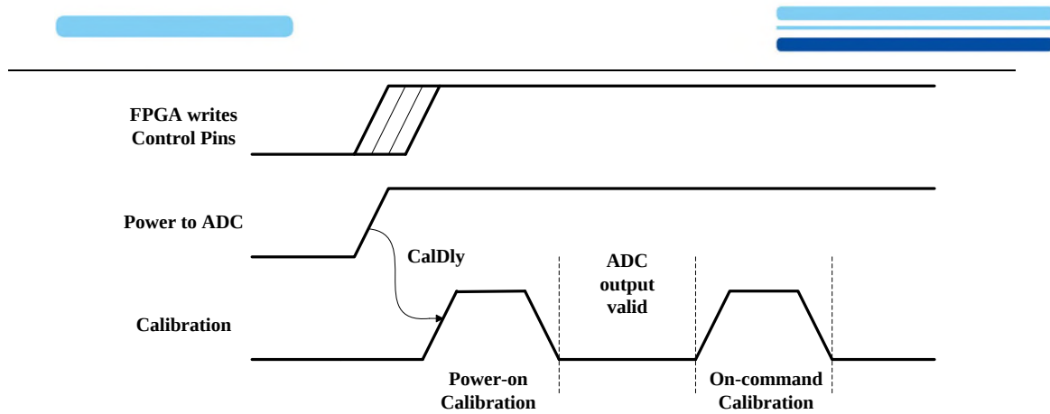
Figure 9-11. Power-on with Control Pins set by FPGA pre Power-on Cal
