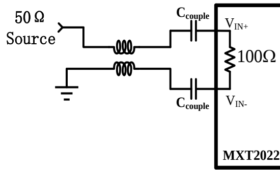
Figure 9-6. Single-Ended to Differential Conversion Using a Balun
