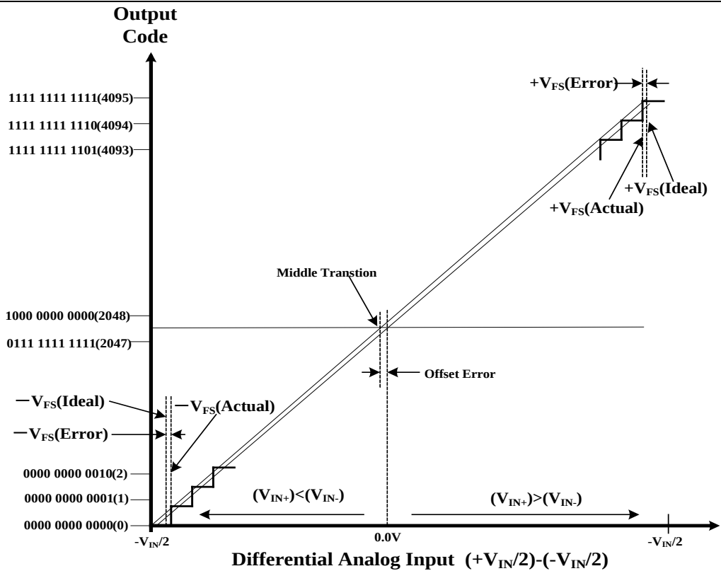
Figure 8-1. Input / Output Transfer Characteristic
