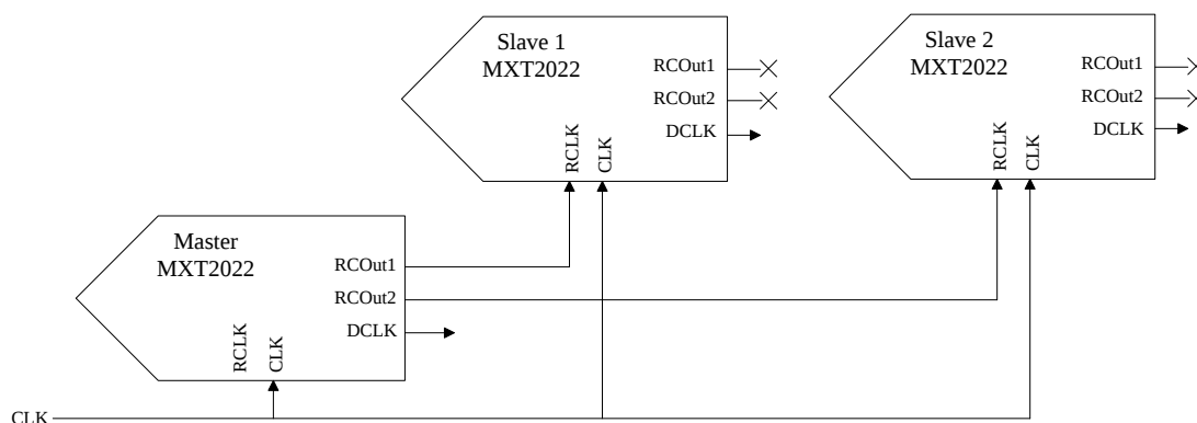
Figure 9-8 AutoSync Example
