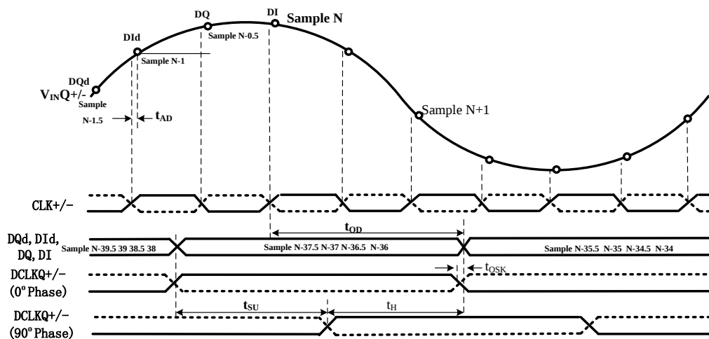
Figure 8-4. Clocking in 1:4 Demux DES Mode
