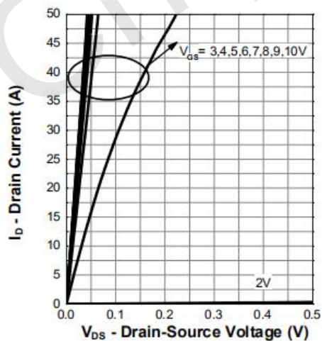
Figure 5. Output Characteristics
