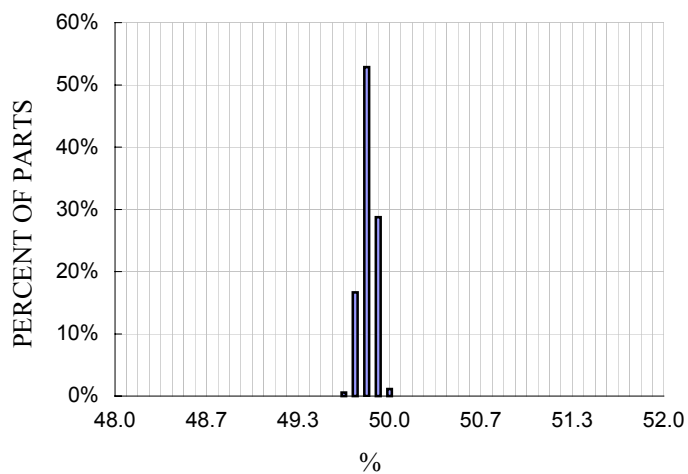
Y-axis Zero g Bias Distribution at Yout, V DD =3V
