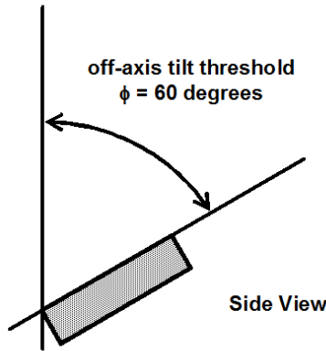
Figure 10: Off-axis tilt
