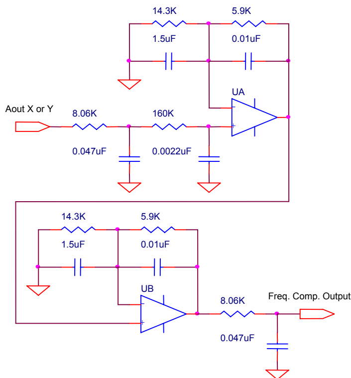
Figure 5: Frequency Response Extension Circuit
