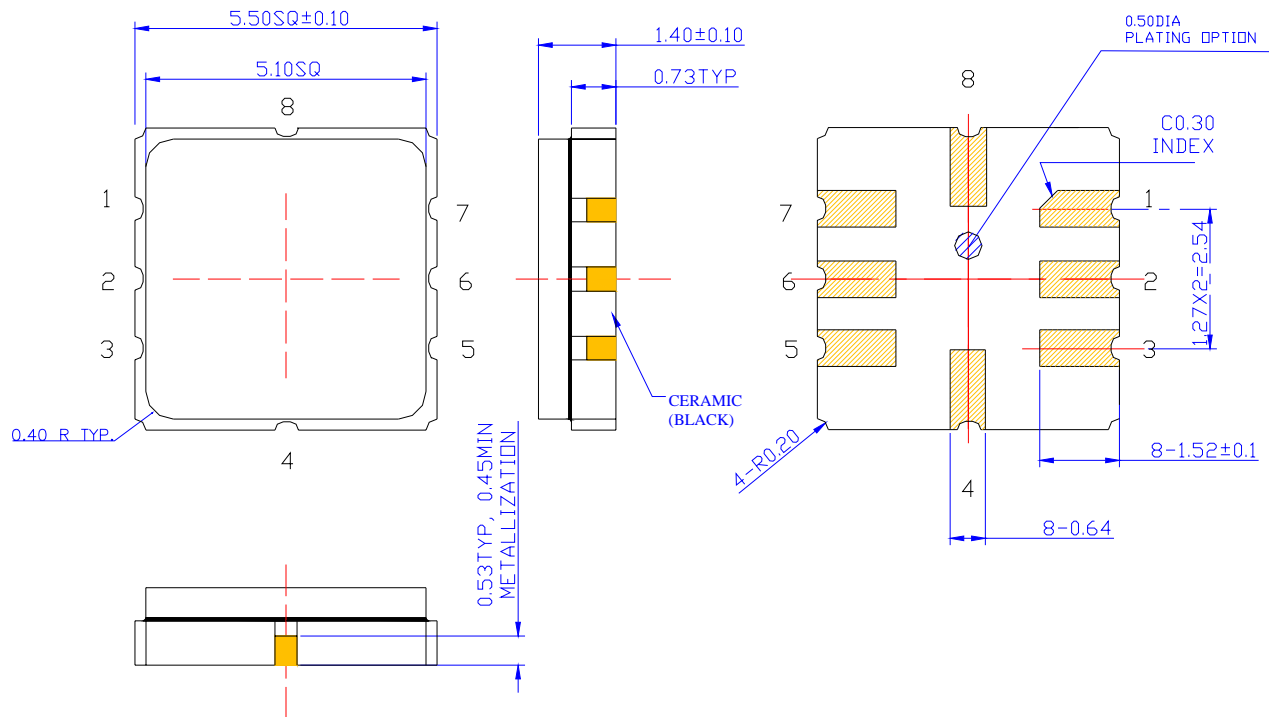
Package Outline
