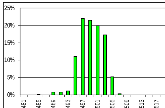
Graph 7. Distribution of AOUTX Sensitivity (mV/g)
