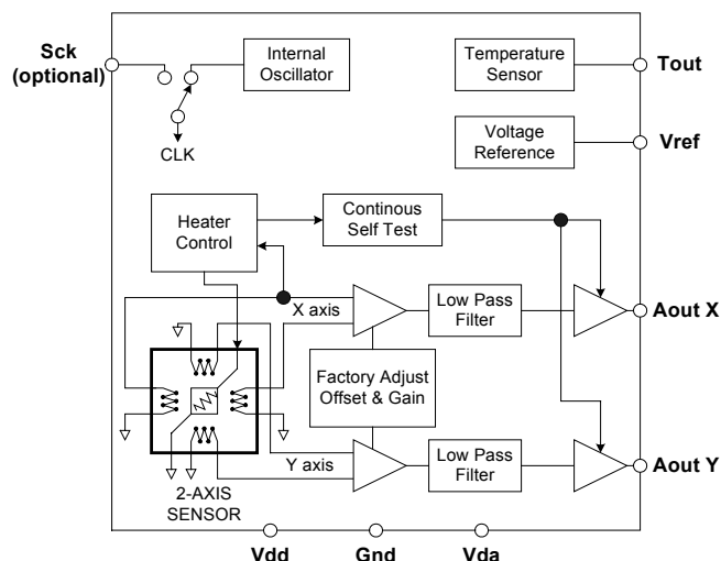
MXA2312A FUNCTIONAL BLOCK DIAGRAM
