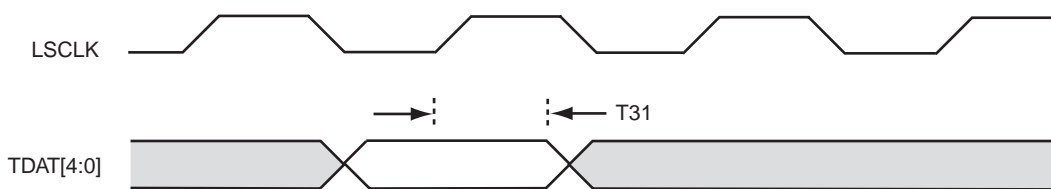
Figure 9-4 Transmit Signal Timing Relationships at the DT
