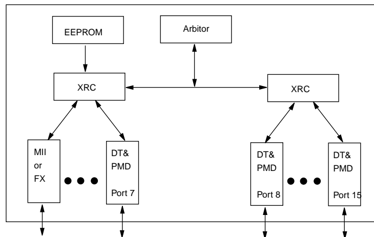
Figure 6-2 TX/MII Mixed Mode operation for XRC II
