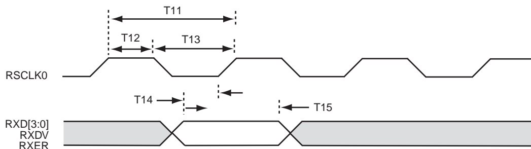
Figure 9-2 Receive Signal Timing Relationships for MII mode
