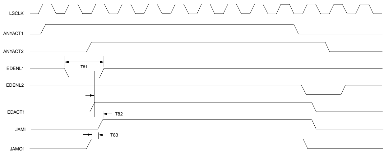
Figure 9-8 Expansion Port with Collision (Note 1)
