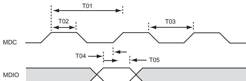
Figure 9-1 MDIO Timing Relationship MDC
