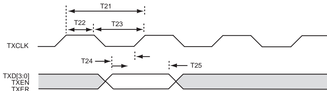
Figure 9-3 Transmit Signal Timing Relationships at the MII
