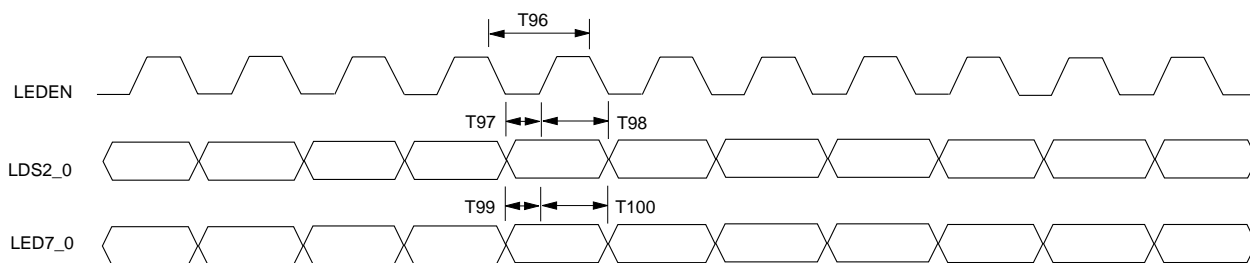
Figure 9-10 Timing Relationship for LED Display
