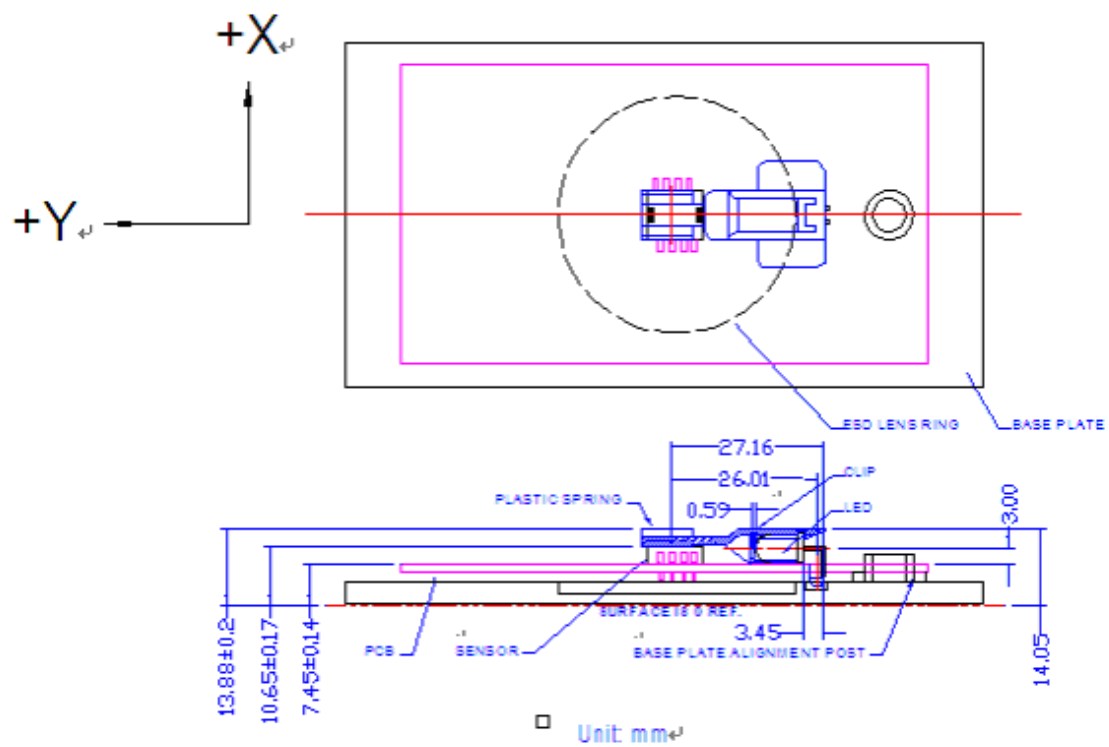
Chart 4 2D Assembly
