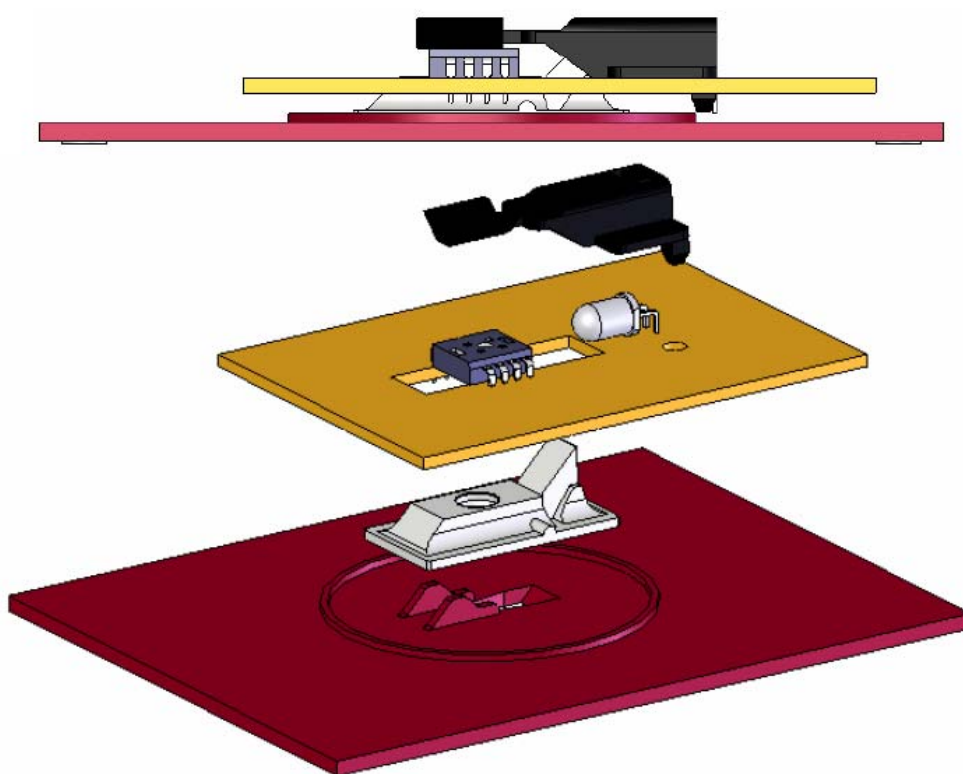
Chart 5 3D Assembly
