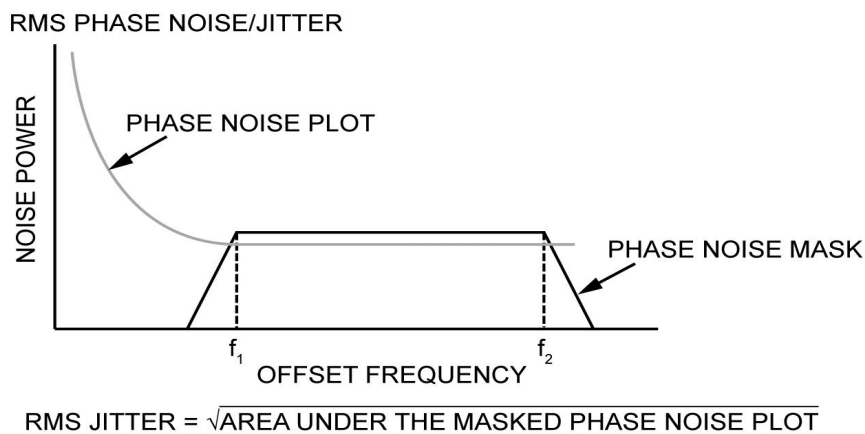
Figure 6. RMS Phase/Noise/Jitter
