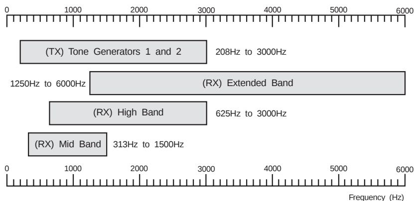
Figure 4: MX803A Frequencies
