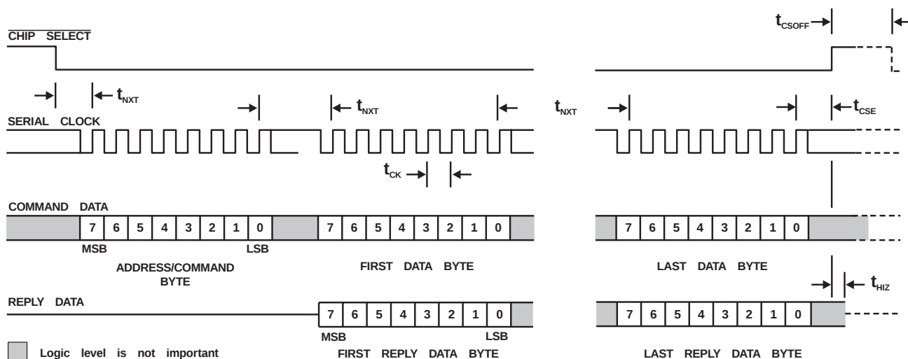
Figure 8: C-BUS Timing
