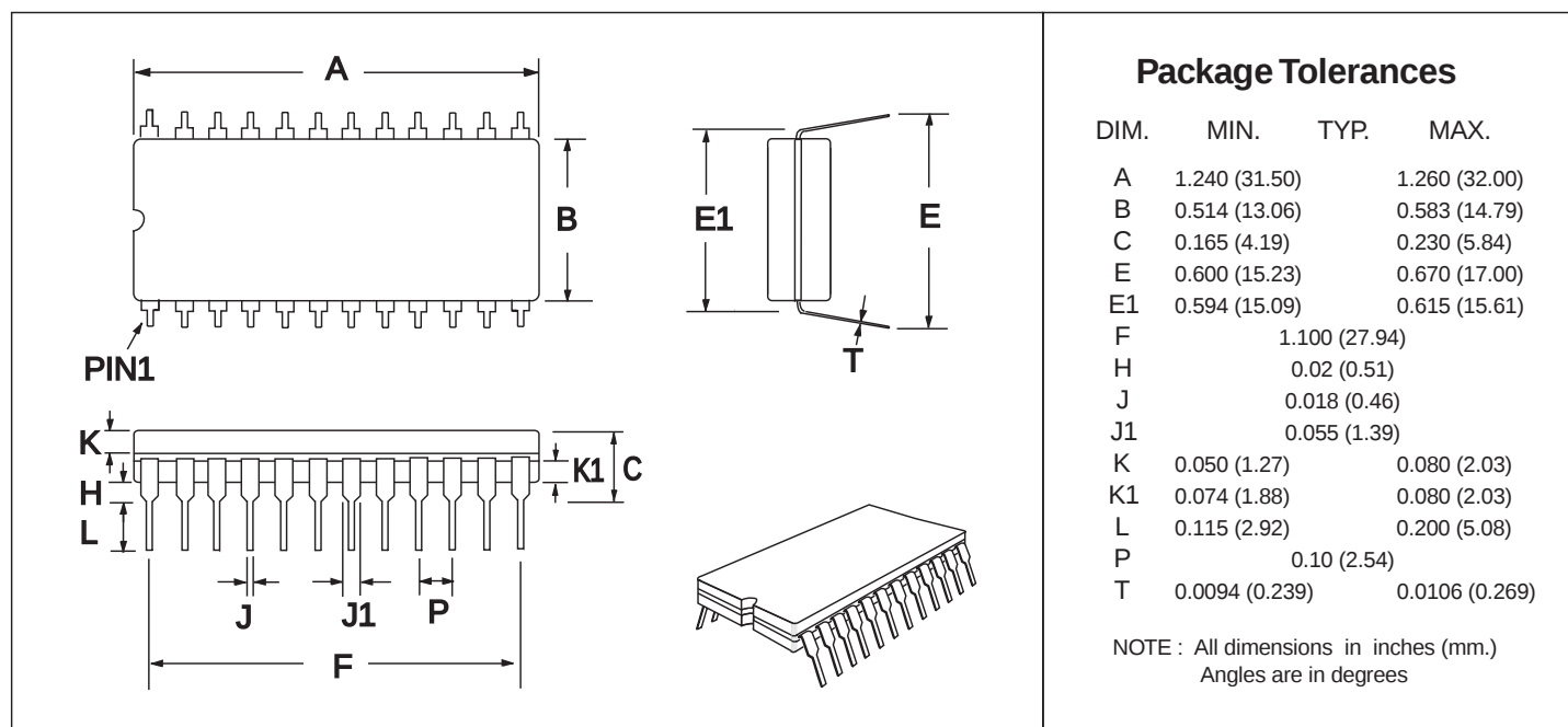
Figure 12: 24-pin CDIP Mechanical Outline: order as part no. MX803AJ
