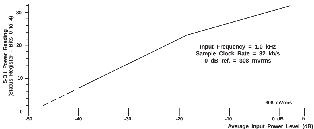
Figure 4: Typical Power Readings vs. Input Levels
