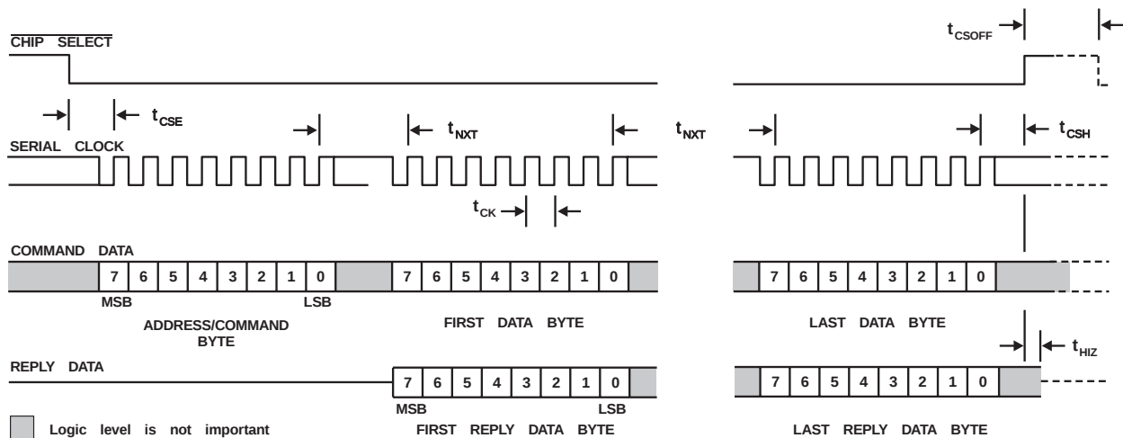
Figure 9: C-BUS Timing Information
