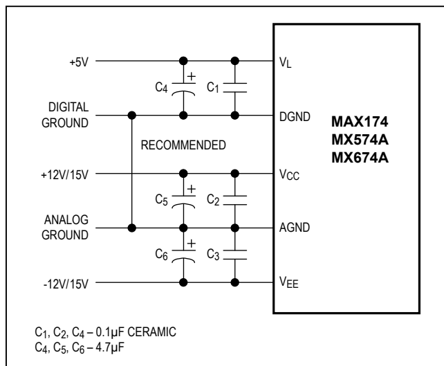
Figure 9. Power-Supply Bypassing
