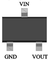
SOT23-3 and SOT23 (Top view)
