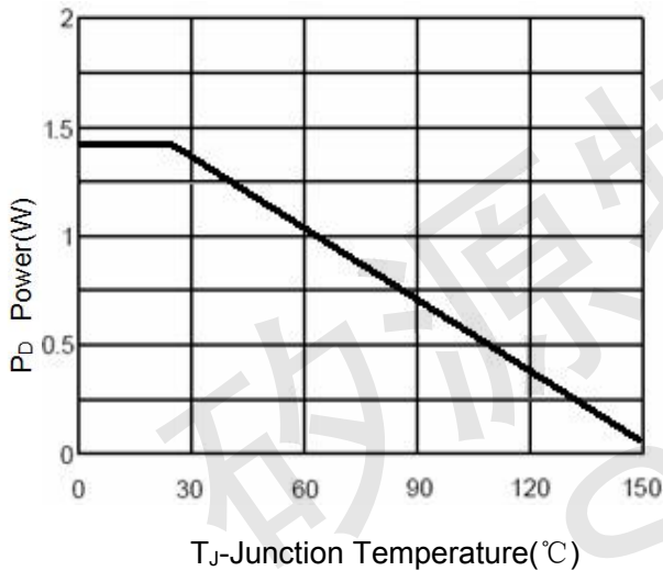
Figure 3 Power Dissipation
