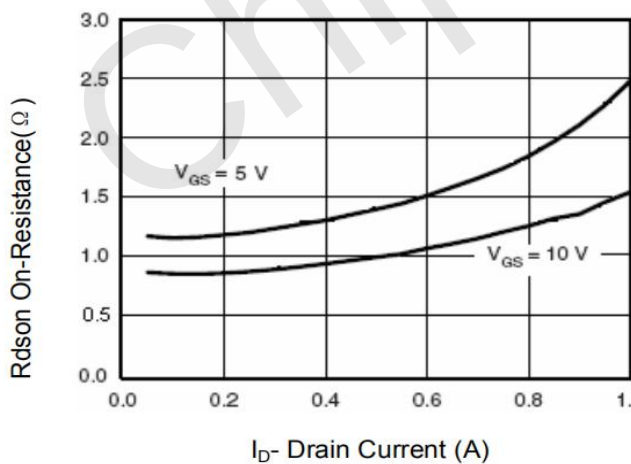
Figure 5 Drain-Source On-Resistance
