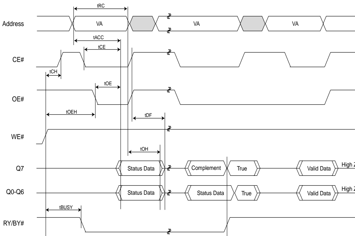
Figure 24. DATA# POLLING TIMING WAVEFORMS (DURING AUTOMATIC ALGORITHMS)
