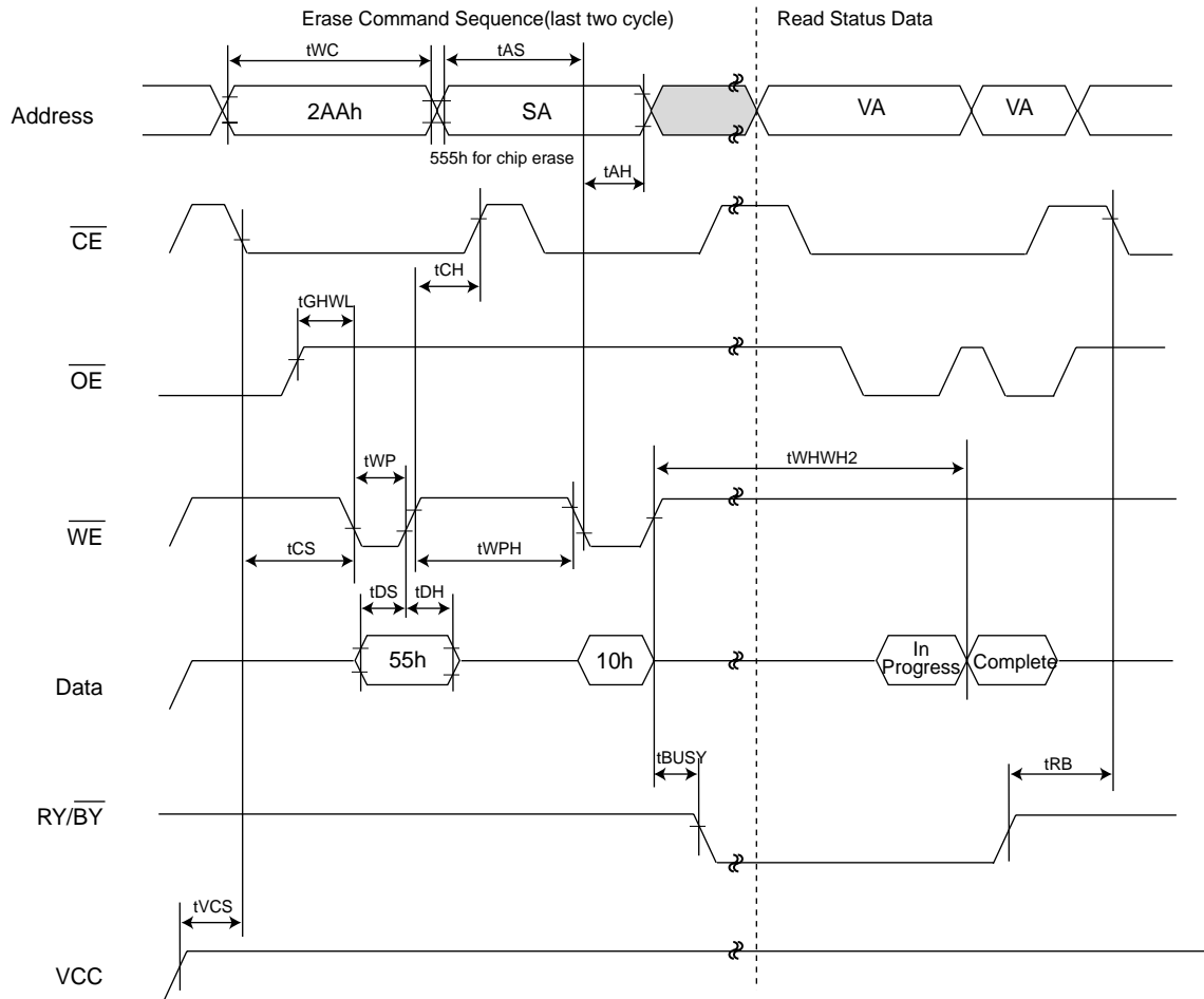
Fig 4. AUTOMATIC CHIP ERASE TIMING WAVEFORM
