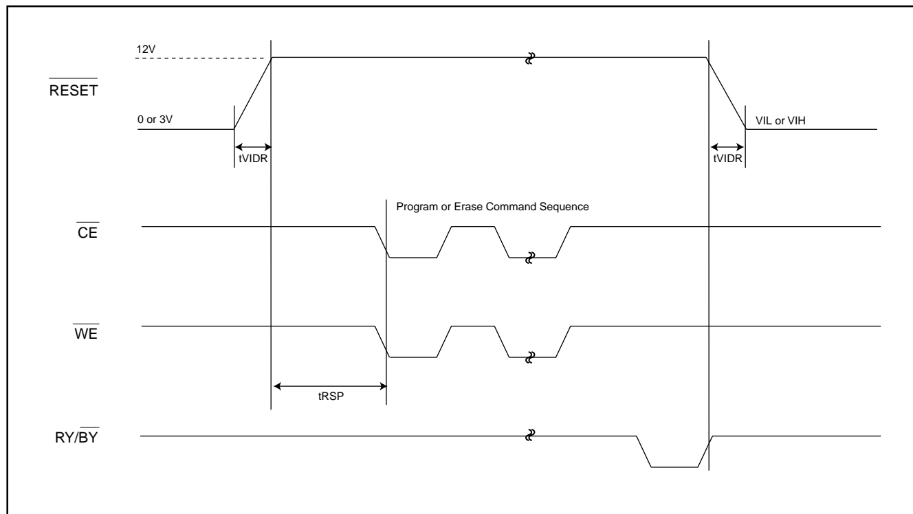
Fig 15. TEMPORARY SECTOR GROUP UNPROTECT WAVEFORMS
