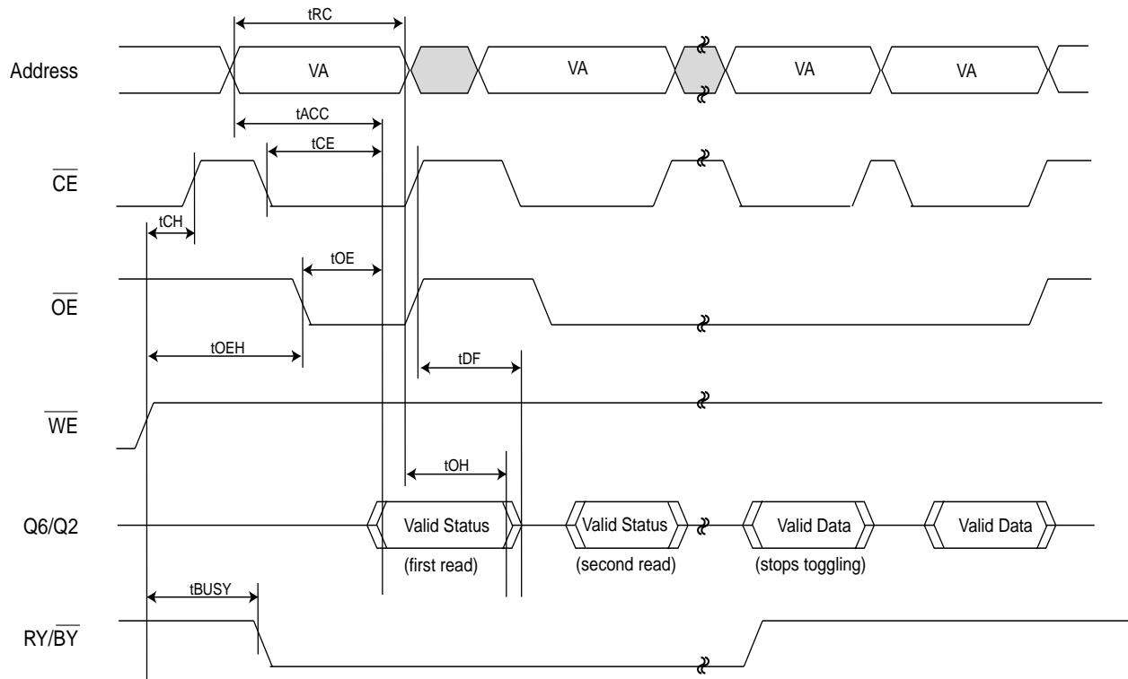
Fig 20. TOGGLE BIT TIMING WAVEFORMS (DURING AUTOMATIC ALGORITHMS)
