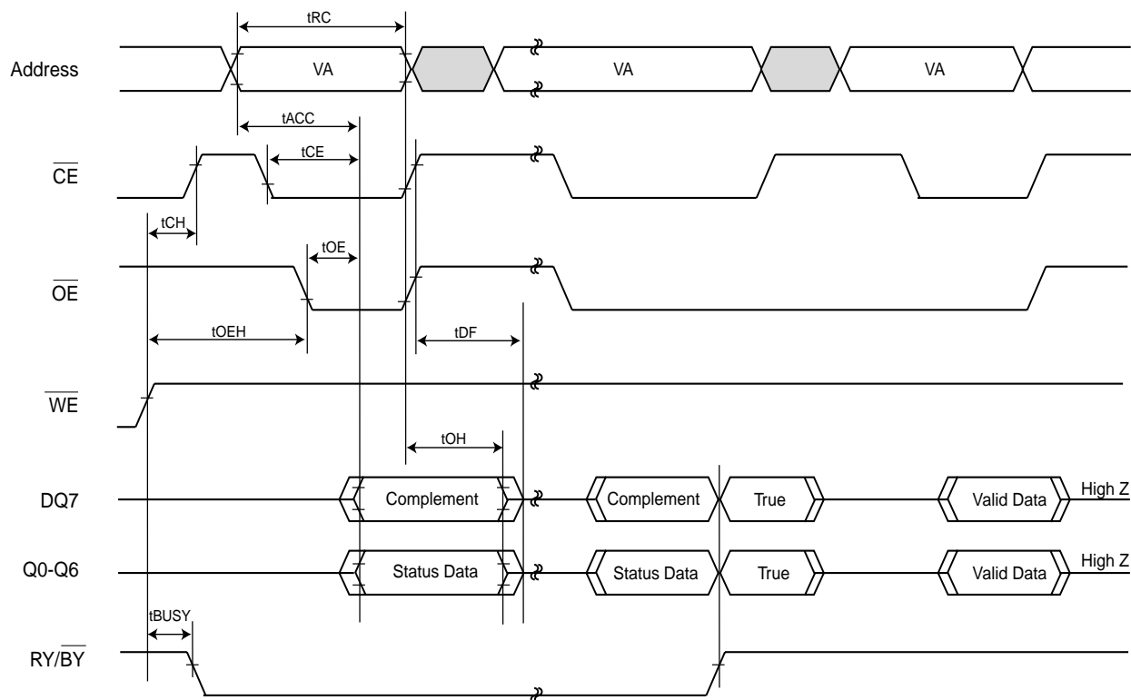
Figure 18. Data Polling Timings (During Automatic Algorithms)
