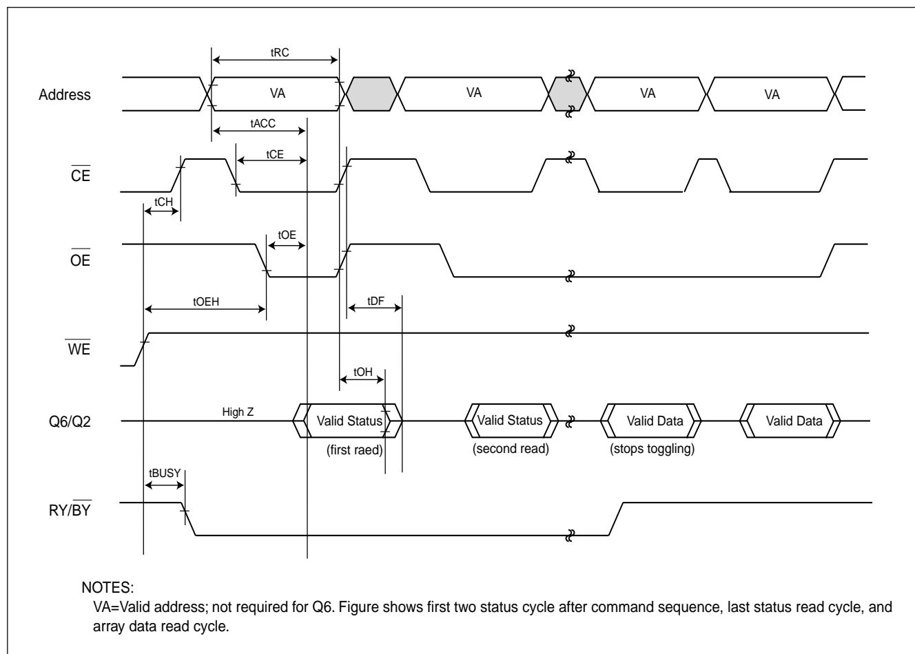
Figure 19. Toggle Bit Timings (During Automatic Algorithms)
