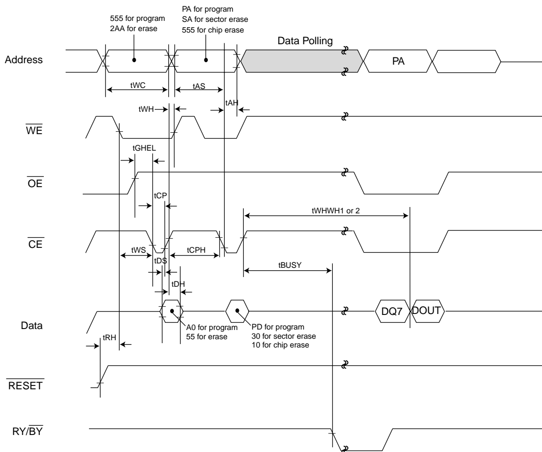
Figure 5. \overline{CE} CONTROLLED PROGRAM TIMING WAVEFORM
