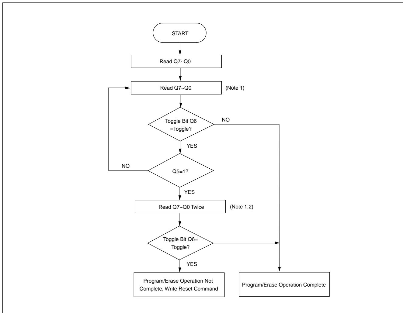
Figure 25. Toggle Bit Algorithm
