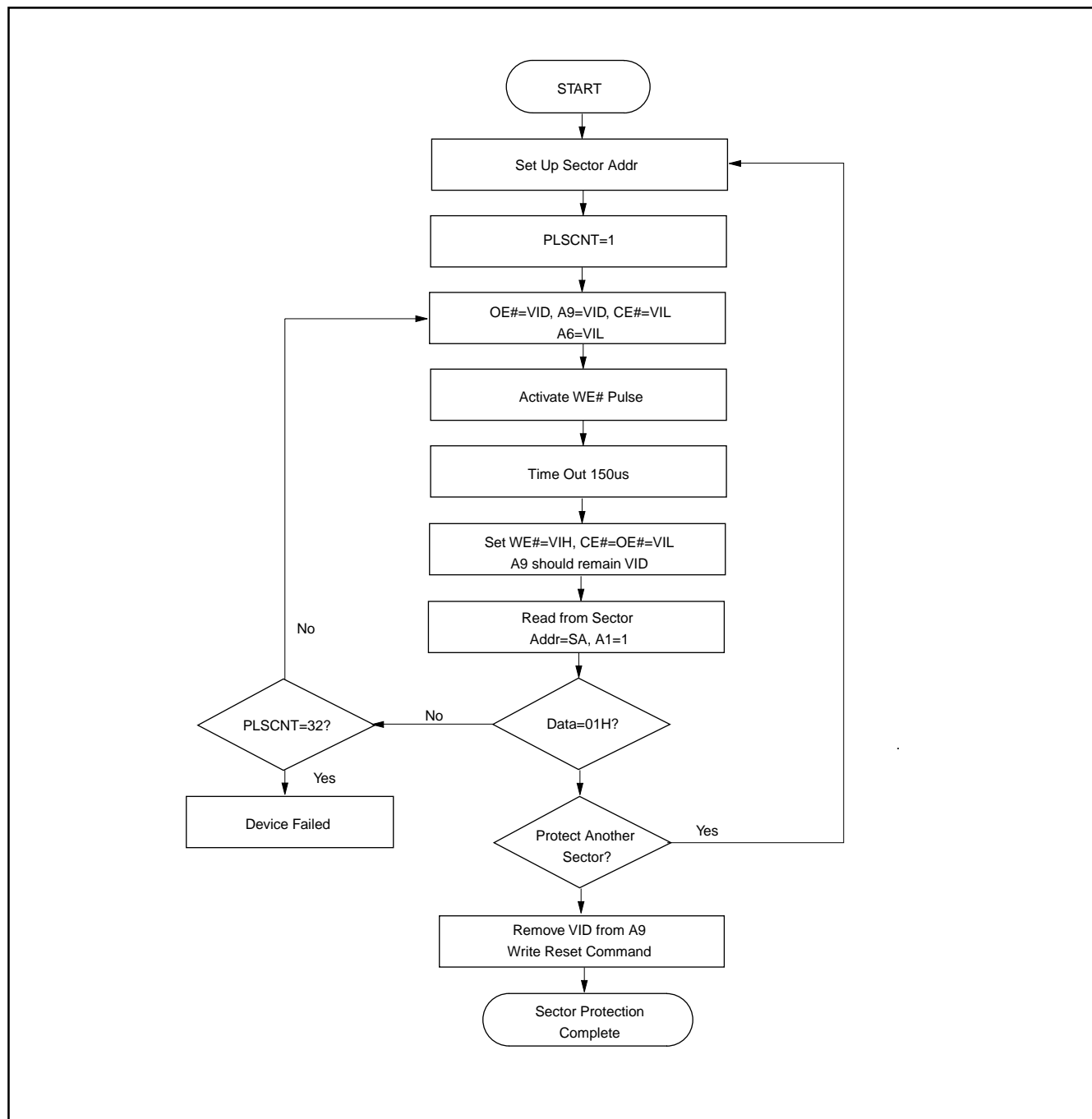
Figure 16. SECTOR GROUP PROTECTION ALGORITHM (A9, OE# Control)
