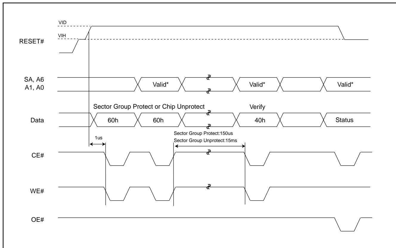
Figure 13. Sector Group Protect / Protect and Unprotected Waveform (RESET# Control)
