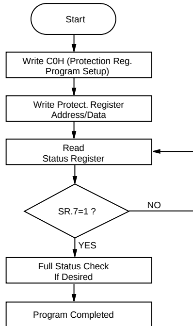
Figure 11. Protection Register Programming Flowchart
