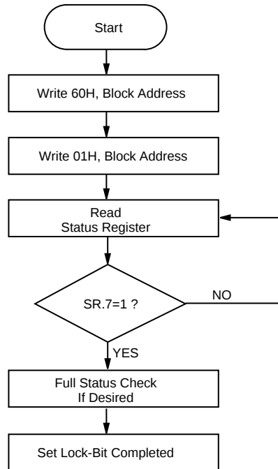
Figure 9. Set Block Lock-Bit Flowchart
