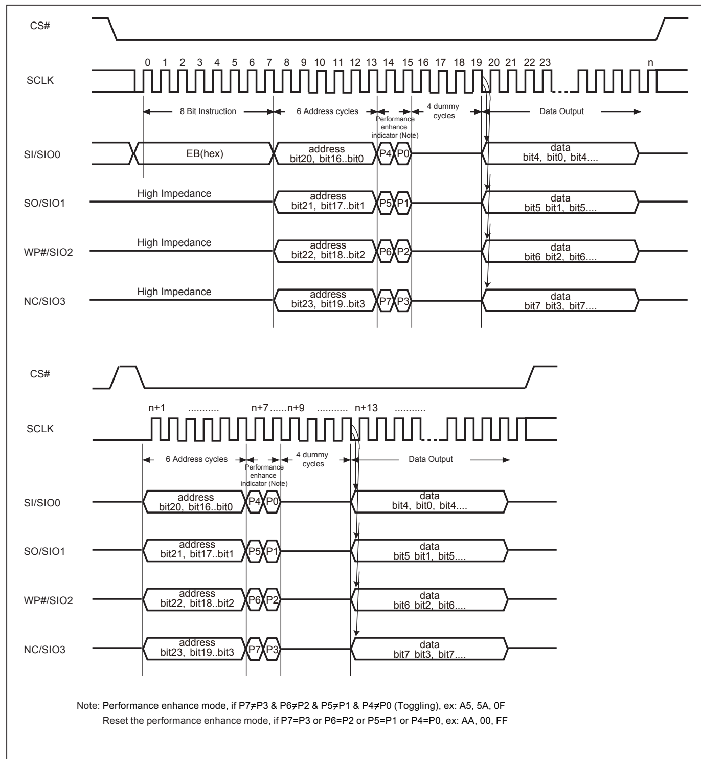
Figure 20. 4 x I/O Read enhance performance Mode Sequence (Command EB)
