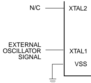
Figure 4. External Clock Drive Configuration
