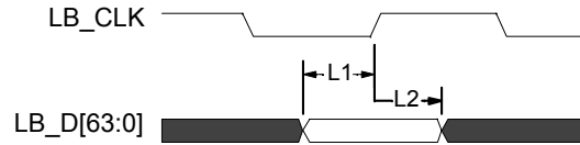
Figure 13 - Local Memory Interface – Input setup and hold timing
