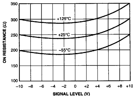
Figure 5. ON Resistance vs. Temperature
