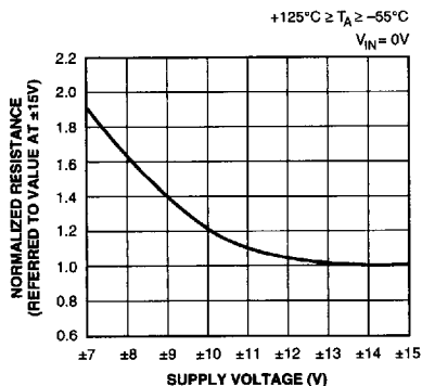
Figure 4. Normalized ON Resistance vs. Supply Voltage
