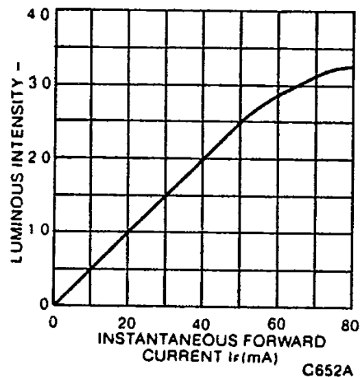
Fig. 2. Luminous Intensity vs. Forward Current
