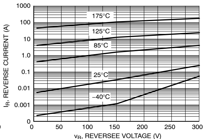
Figure 4. Typical Reverse Voltage
