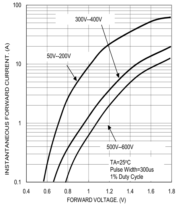
FIG. 5- TYPICAL FORWARD CHARACTERISTICS
