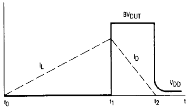
Figure 7. Current-Voltage Waveforms
