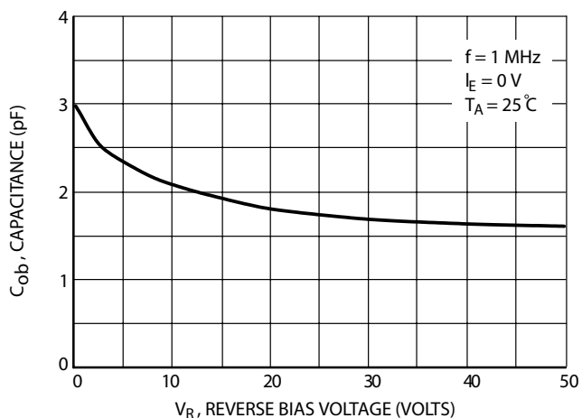
FIG.9 Output Capacitance
