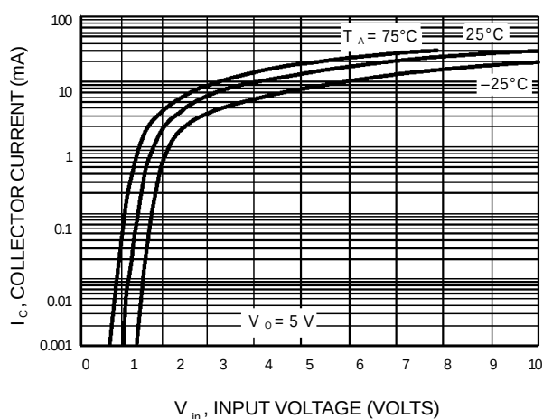
Figure 15. Output Current versus Input Voltage
