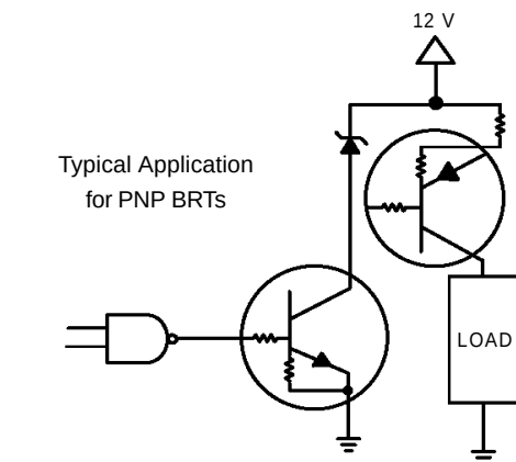
Figure 22. Inexpensive, Unregulated Current Source
