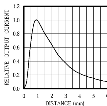
I_o VS DISTANCE
