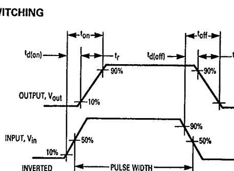
Figure 14. Switching Waveforms
