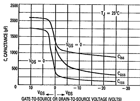
Figure 11. Capacitance Variation
