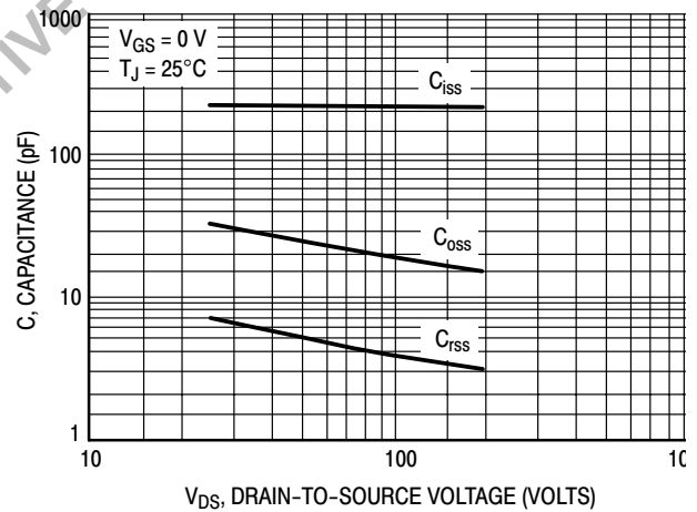
Figure 1b. High Voltage Capacitance Variation
