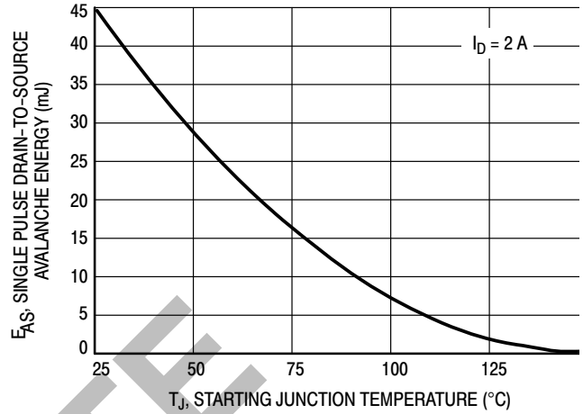
Figure 11. Maximum Avalanche Energy versus Starting Junction Temperature
