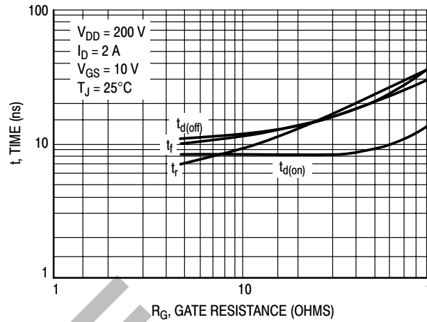
Figure 8. Resistive Switching Time Variation versus Gate Resistance
