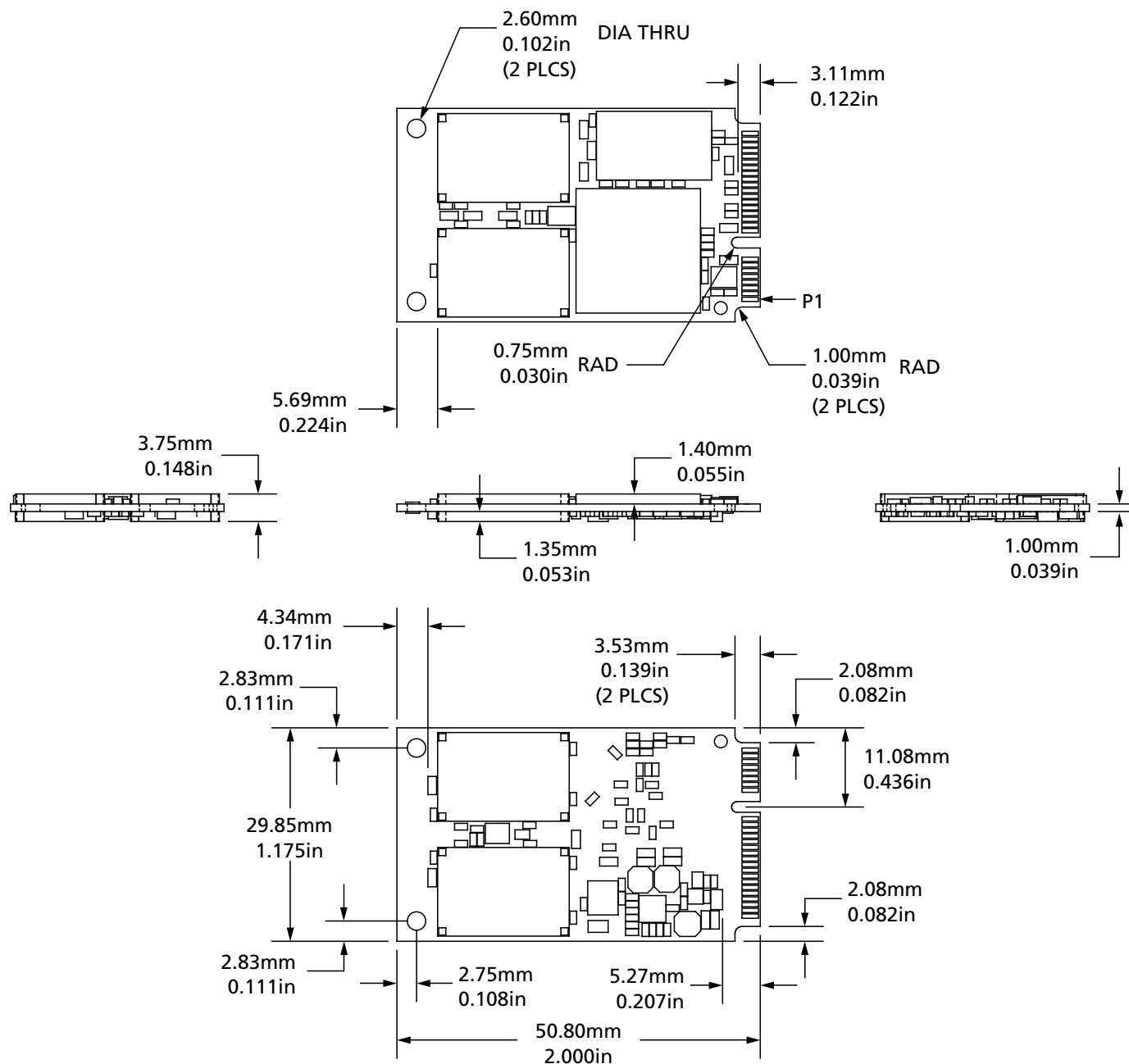
Figure 4: mSATA Package – 50.80mm
