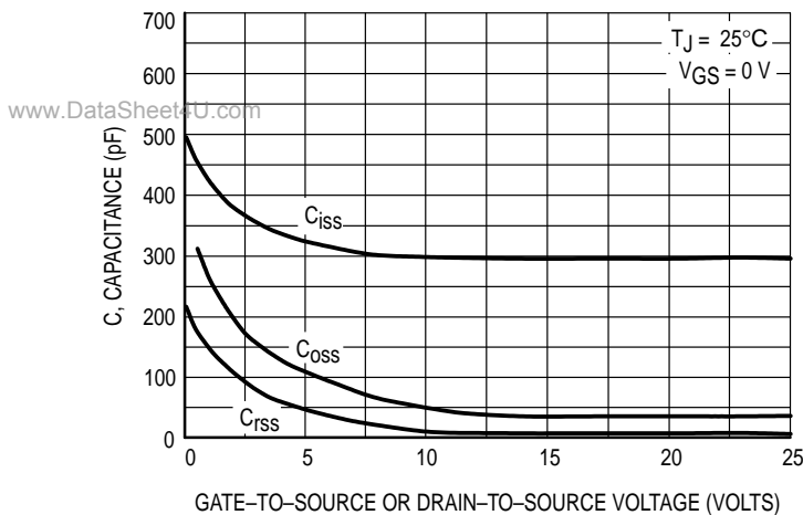
Figure 7a. Capacitance Variation
