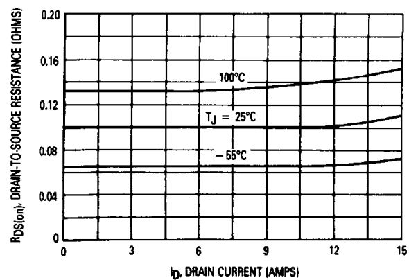
Figure 6. On-Resistance versus Drain Current
