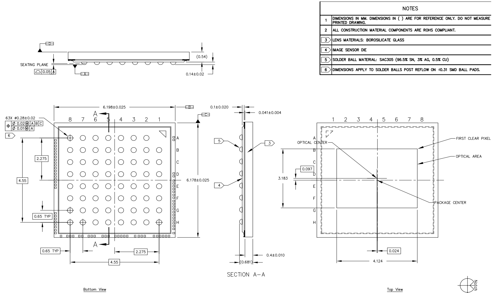
Figure 57: 63-Ball CSP Package Outline Drawing
