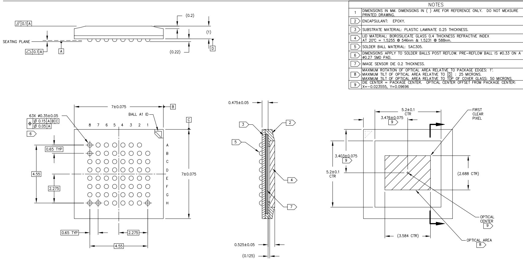
Figure 56: 63-Ball cBGA Package Outline Drawing
