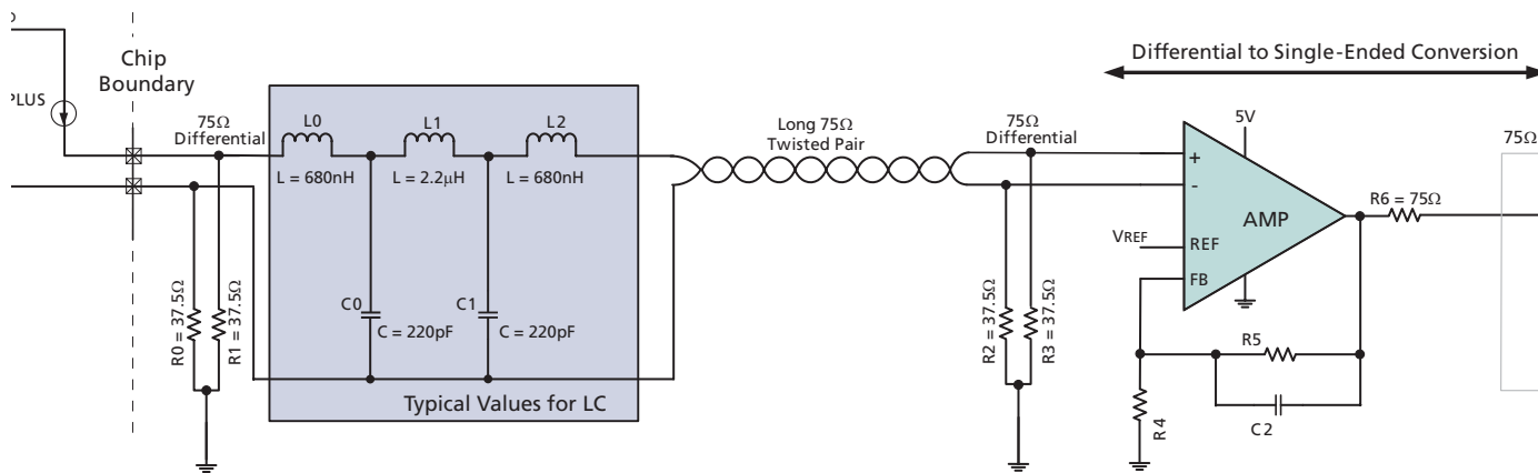
Figure 22: Differential Connection—Grounded Terminations
