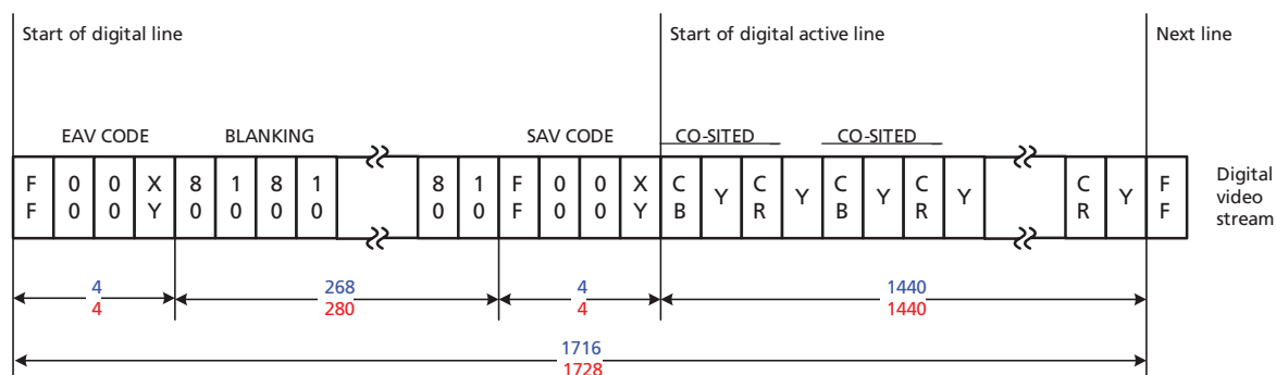
Figure 25: CCIR656 8-Bit Parallel Interface Format for 525/60 (625/50) Video Systems
