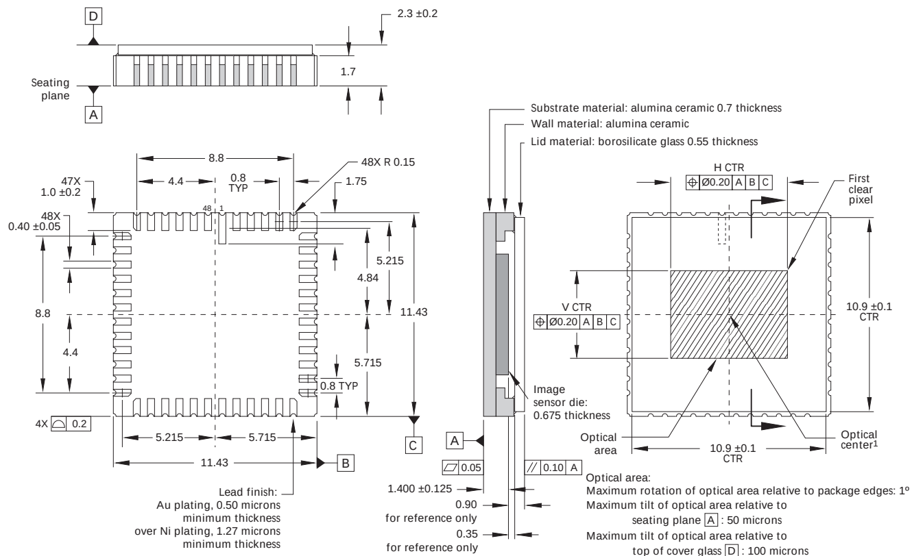
Figure 32: 48-Pin CLCC Package Drawing
