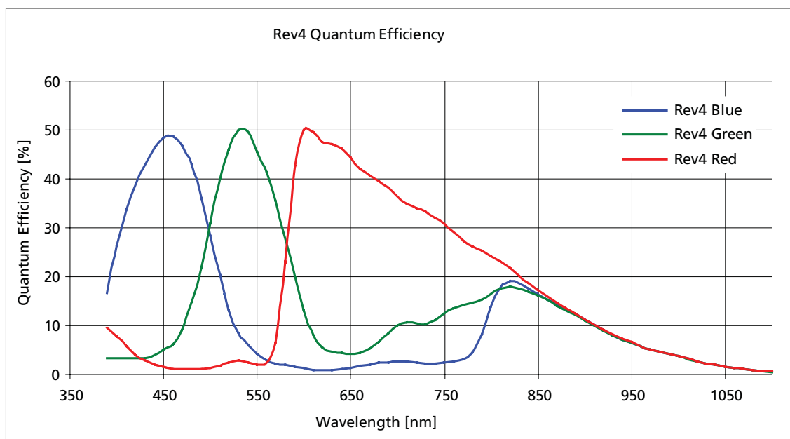
Figure 31: Spectral Characteristics
