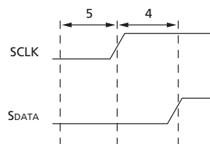
Figure 39: Serial Host Interface Stop Condition Timing
