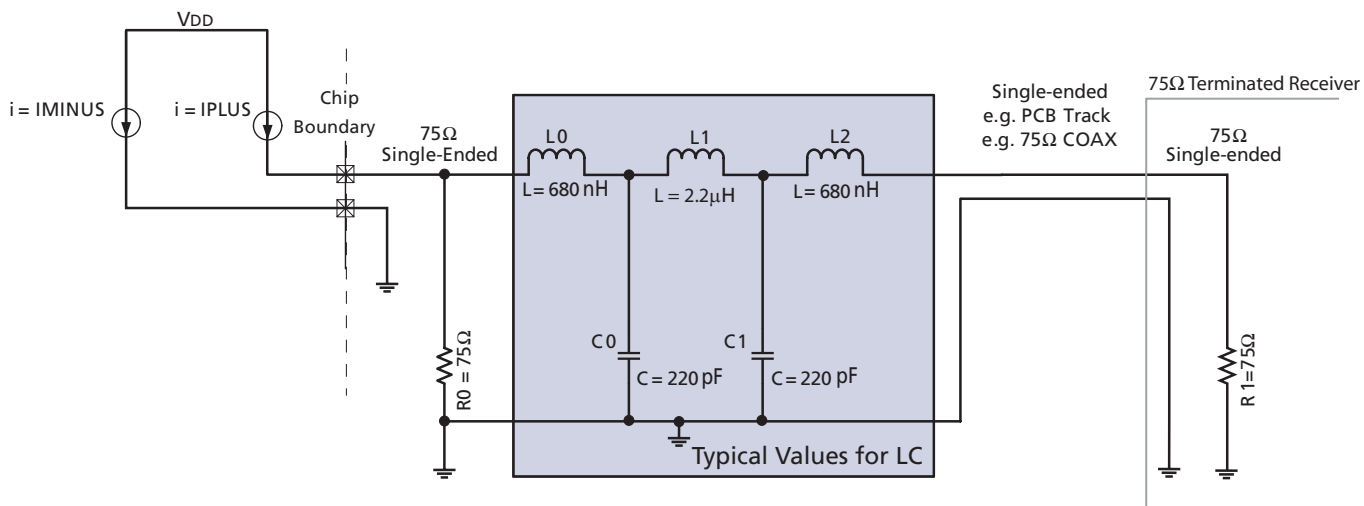
Figure 20: Single-Ended Termination
