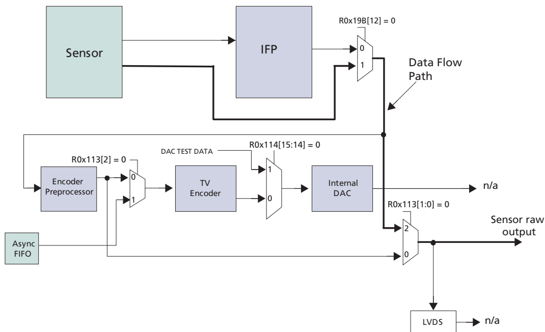
Figure 12: MT9V135 in Sensor Stand-Alone Mode
