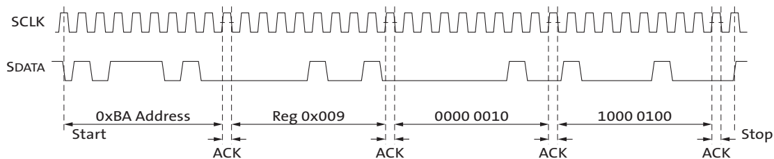
Figure 36: WRITE Timing to R0x009—Value 0x0284
