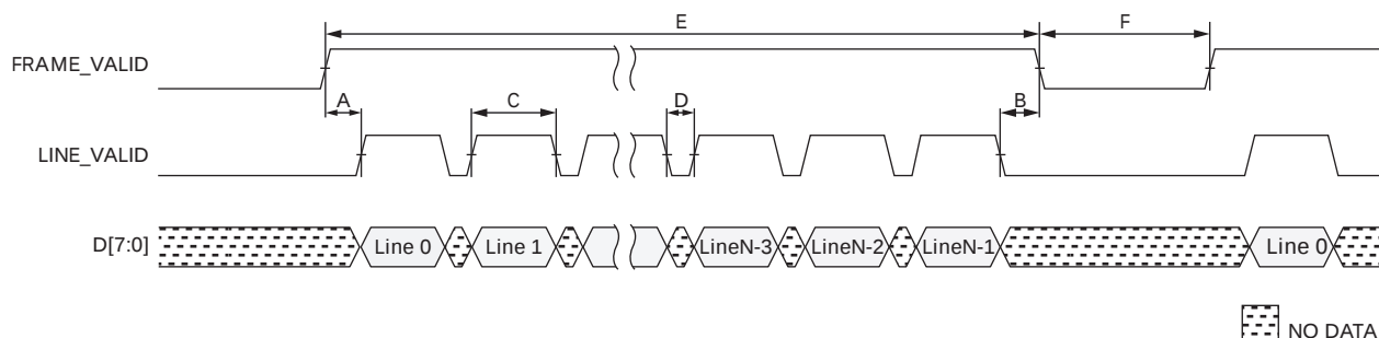
Figure 10: Vertical Timing
