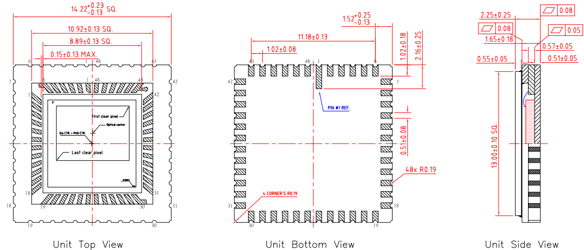
Figure 25: 48-Pin CLCC
