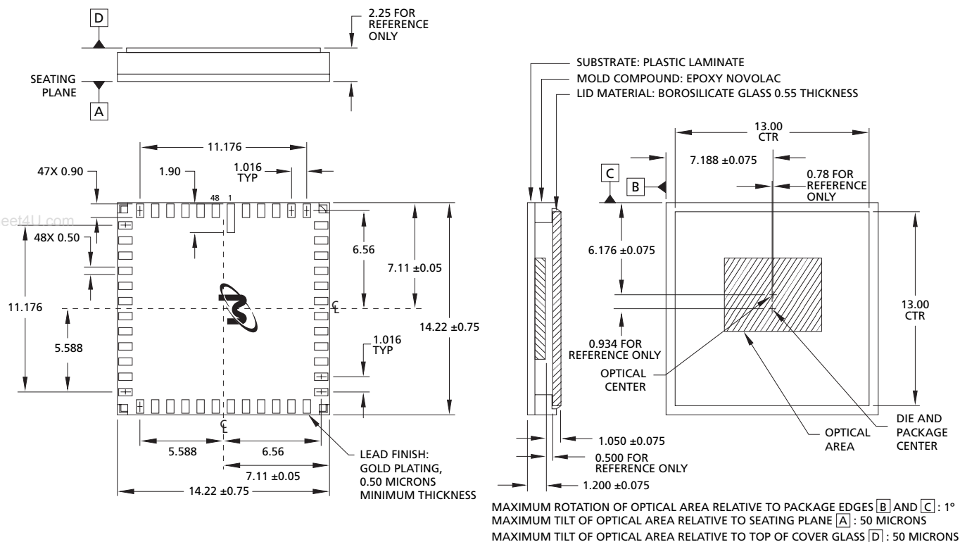
Figure 30: 48-Pin PLCC
