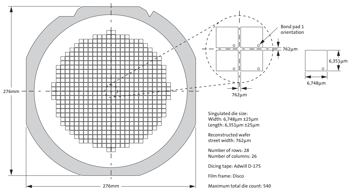
Figure 3: Die Orientation in Reconstructed Wafer
