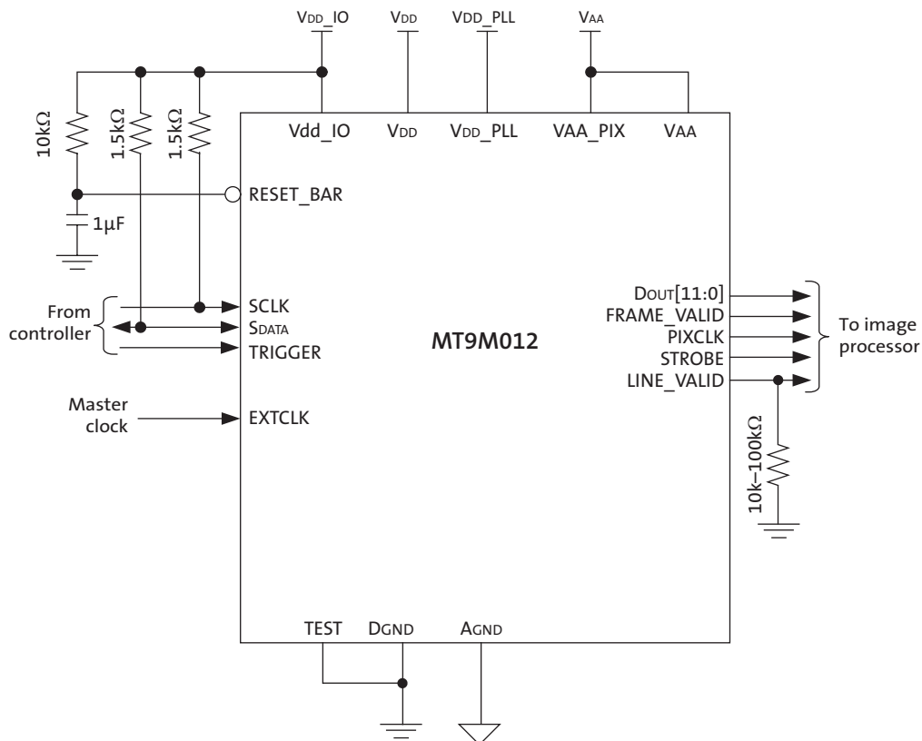
Figure 1: Typical Configuration (Connection) Parallel Mode
