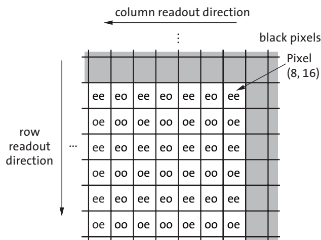
Figure 4: Pixel Pattern Detail (Top Right Corner)
