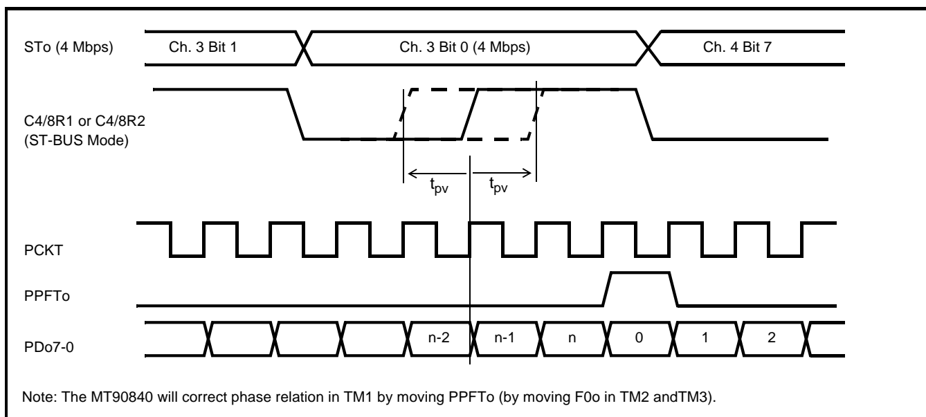
Figure 30 - Phase Variation Between C4/8R1 &amp; C4/8R2 and PCKT Inputs for TM1 Operation
