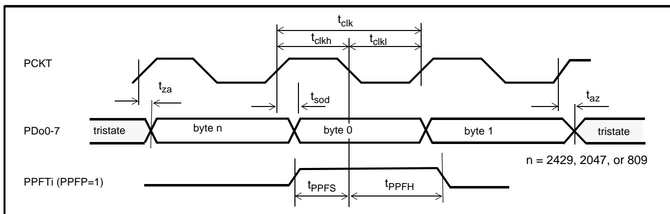
Figure 26 - TM1 Parallel Port Transmit Timing (TM1 &amp; PFDI = 1, PPFT is an input)
