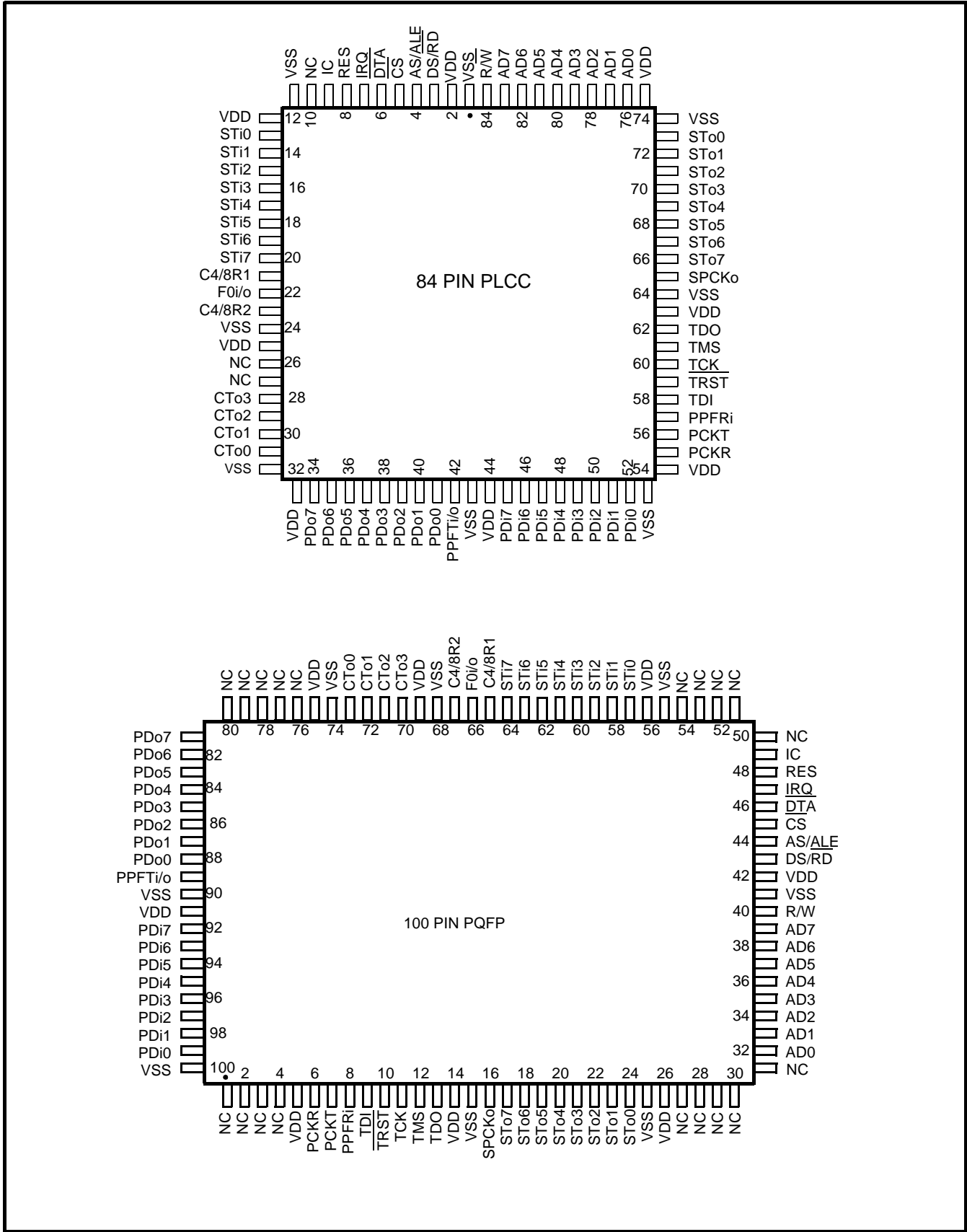
Figure 2 - Pin Connections
