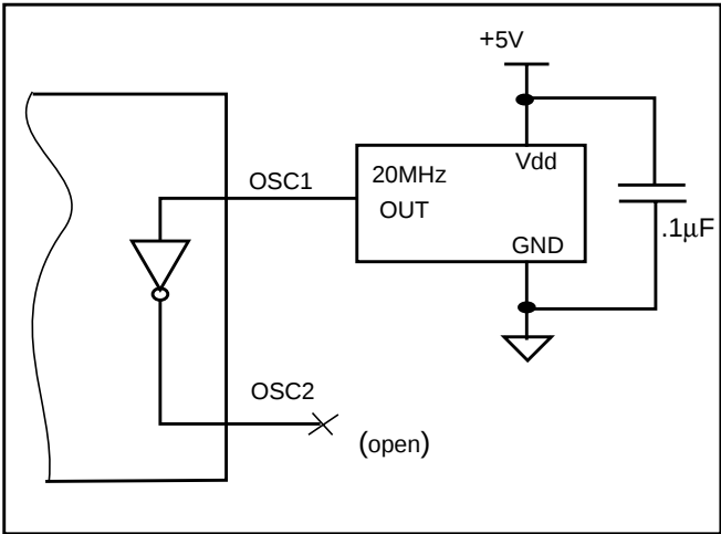
Figure 9 - Clock Oscillator Circuit
