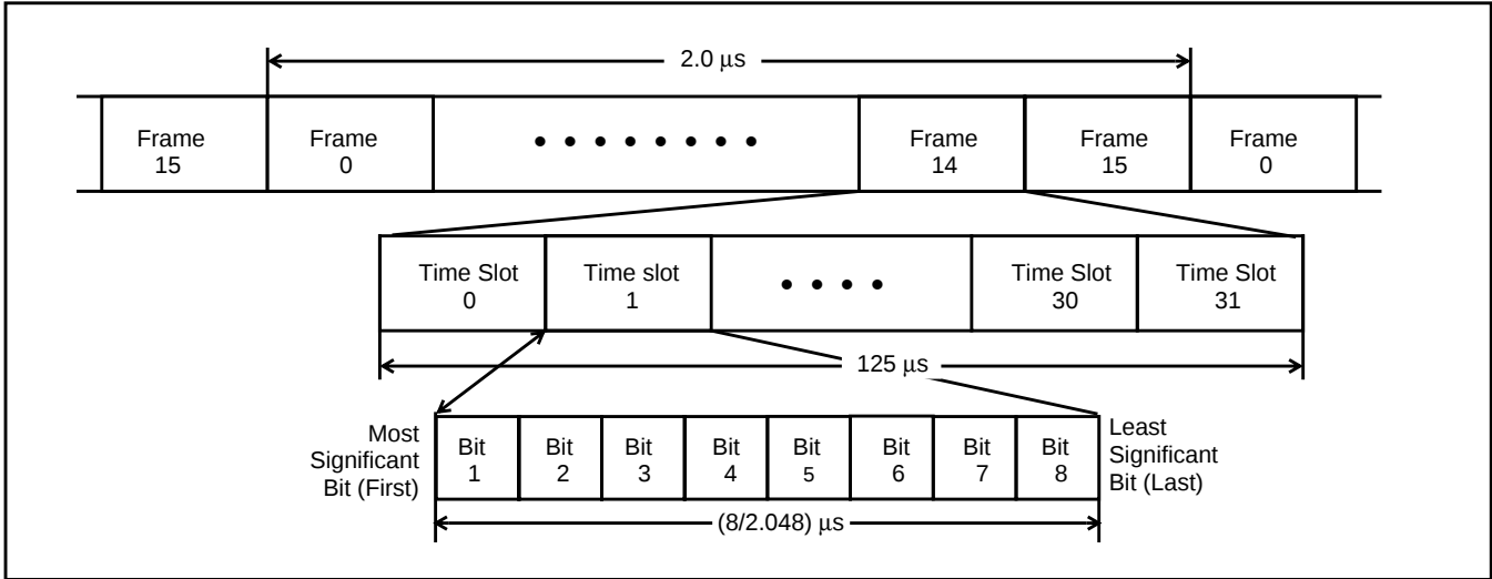
Figure 34 - PCM 30 Format
