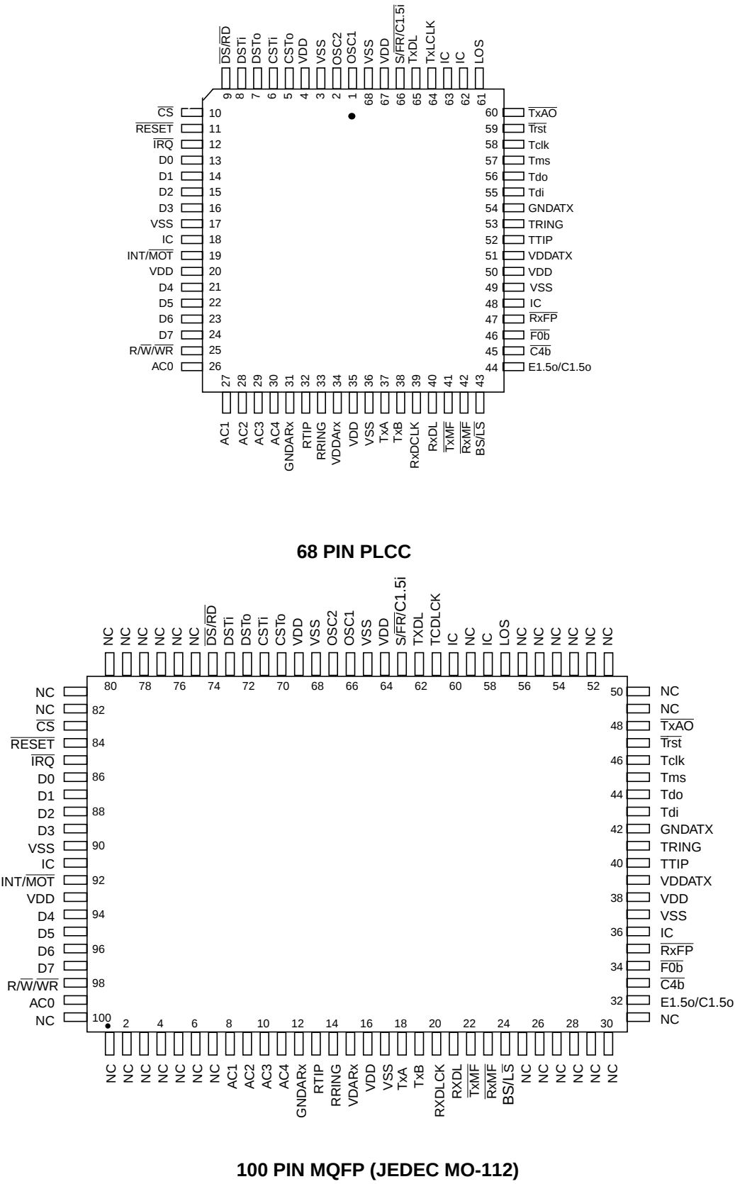
Figure 2 - Pin Connections
