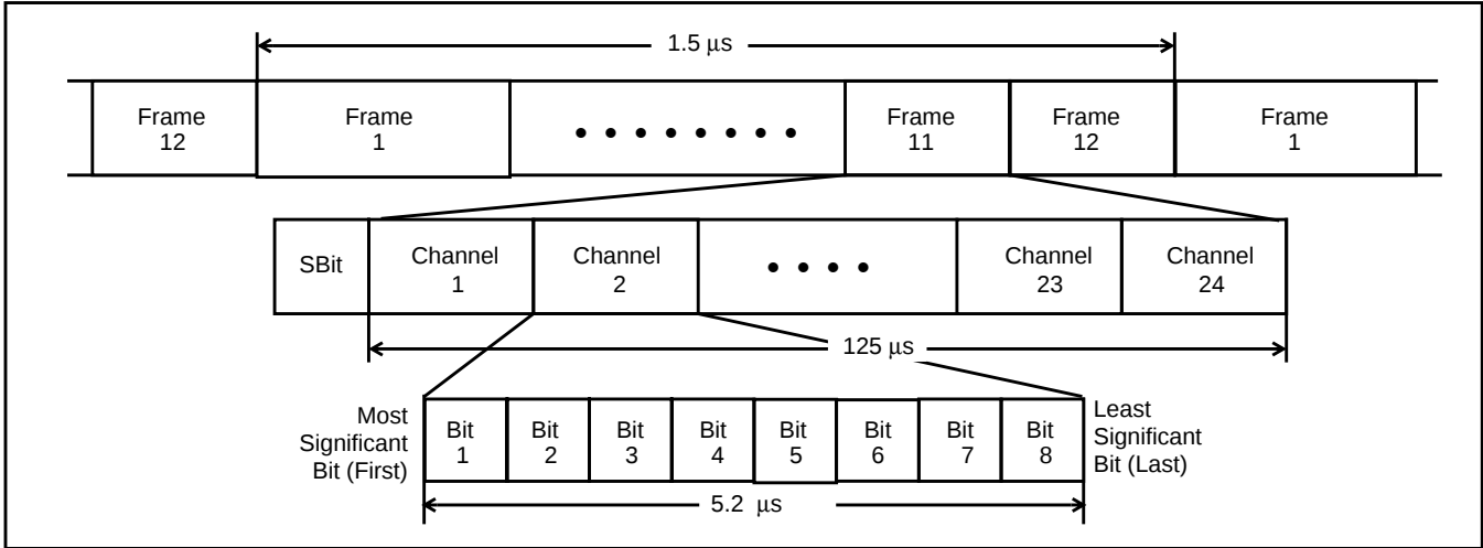
Figure 33 - D4 Format
