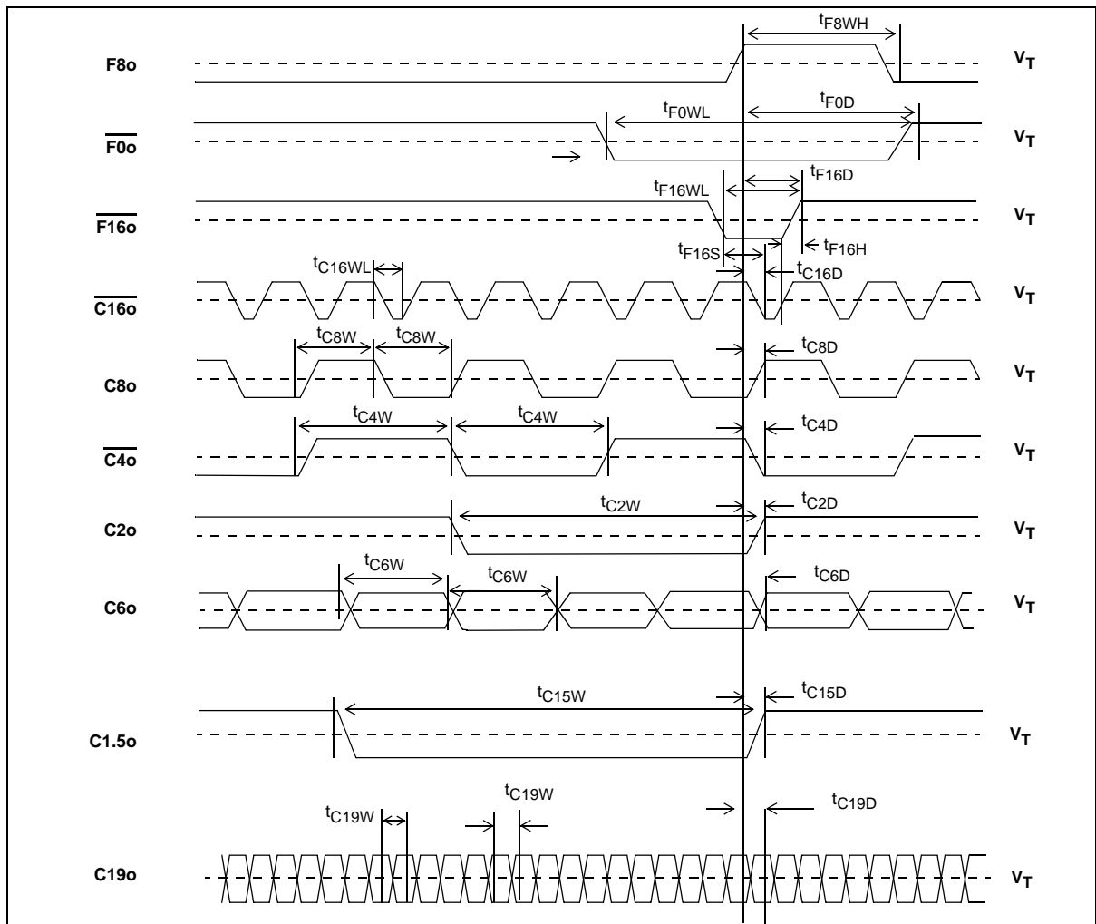
Figure 15 - Output Timing 1
