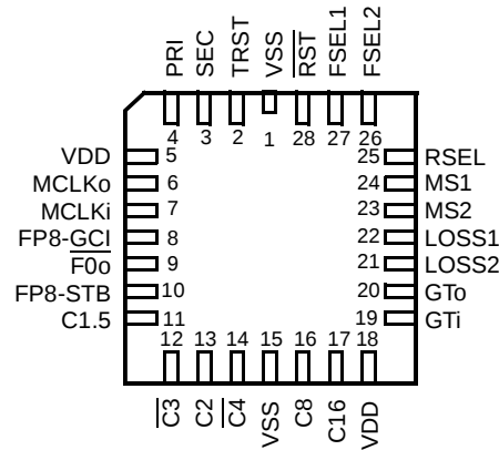
Figure 2 - Pin Connections
